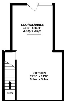
NEW FLOOR 266 sq.ft. (24.7 sq.m.) approx.
